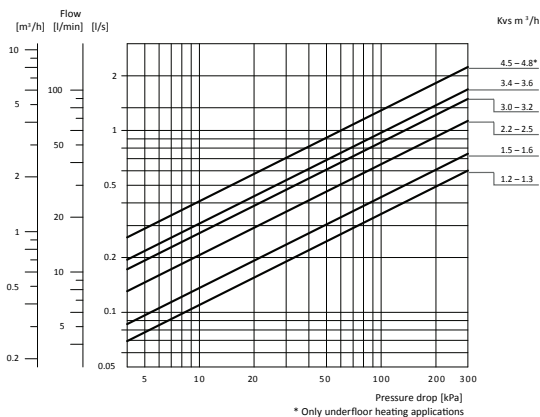
CAPACITY DIAGRAM
