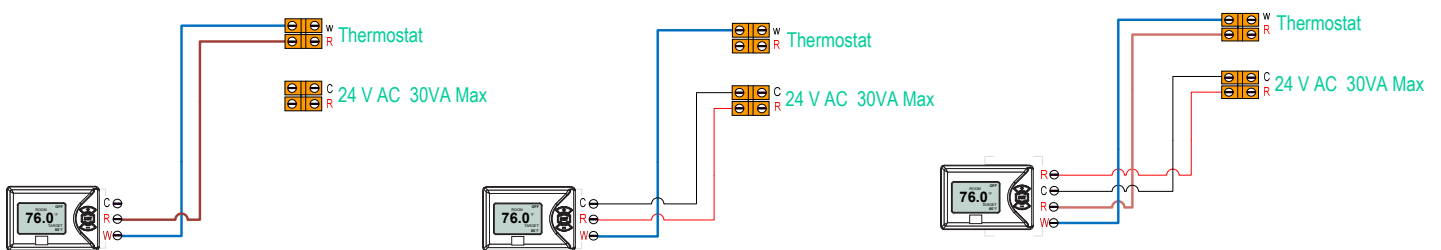
2 Wire Thermostat
