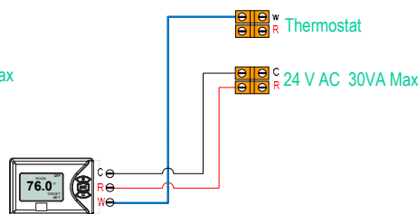
3 Wire Thermostat
