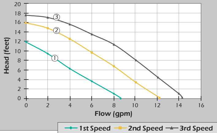
Pump Performance Curve UPS-15-58
