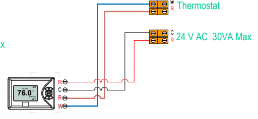
4 Wire Thermostat
