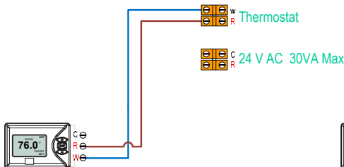
2 Wire Thermostat
